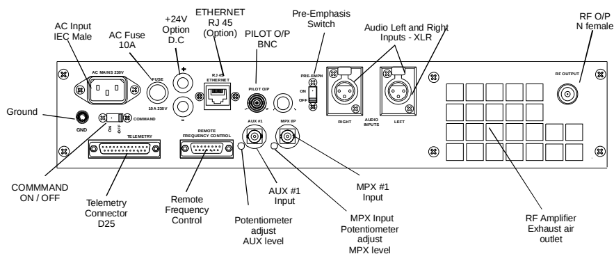
EX-150LD 150W FM TRANSMITTER REAR PANEL
