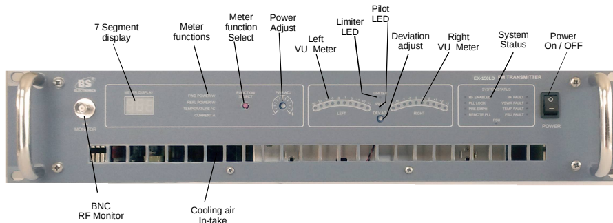
EX-150LD 150W FM TRANSMITTER FRONT PANEL
